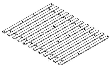
21 (1961x50x18mm) x 12
