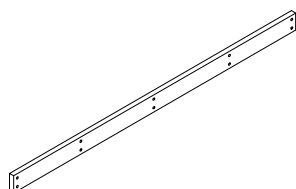
13 (1690x80x22mm) x 1
