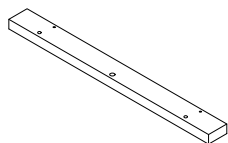
1 (437X40X15mm)X1
