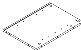
3 (477X337X15mm)X1
