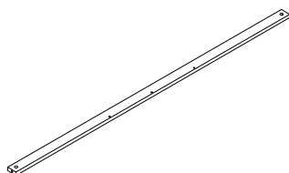
6 (1658X50X18mm)X1
