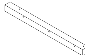
8 (585X40X40mm)X1
