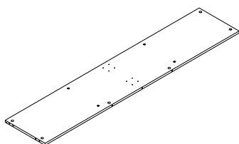
5 (1658X340X15mm)X1
