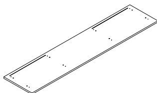
14 (1778X395X18mm)X1
