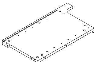
10 (585X320X33mm)X1
