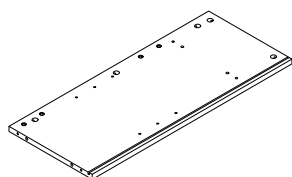
5 (708X295X15mm)X1
