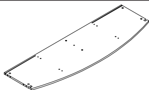
1 (1406X445X15mm)X1
