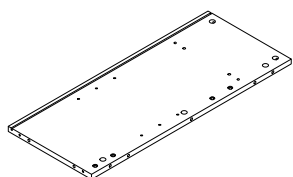
6 (708X295X15mm)X1
