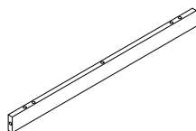
13 (684X49X15mm)x1
