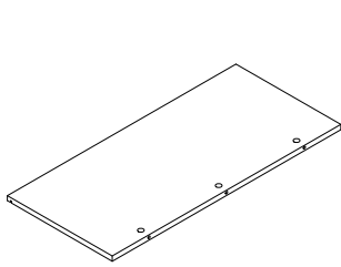
1 (752X345X15mm)X1
