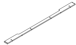
12 (1570X75X15mm)X1
