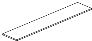
2 (1572*298*18mm x1)
