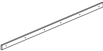
25 (1181*40*12mm x1)
